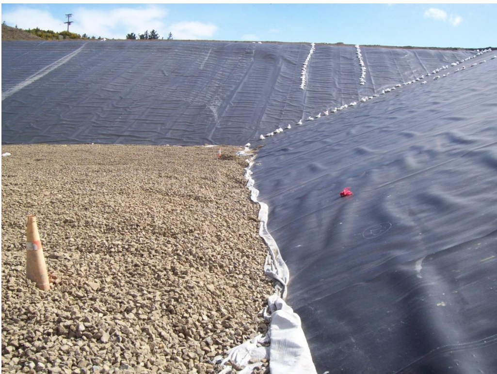
Photograph 17: Stage 2 liner completed
