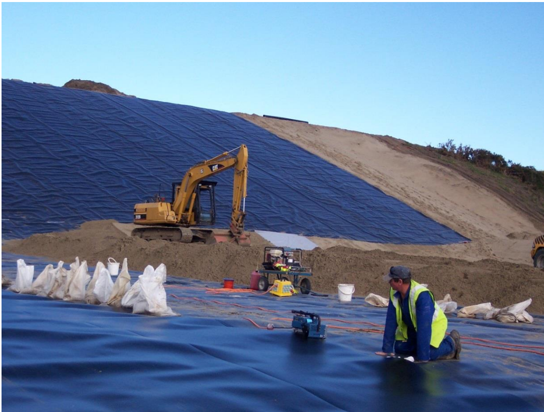
Photograph 11: Placement of sand protection layer Stage 1A (2004)
