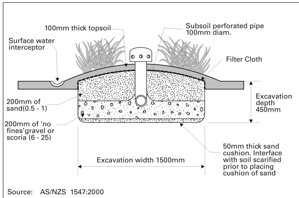
Figure 6.5 Typical Evapotranspiration Seepage Bed Detail
