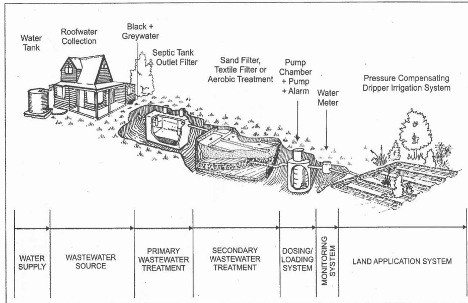
Figure 1.2 Process-flow schematic for on-site wastewater system components. (Source: Auckland Regional Council TP58 2004).
