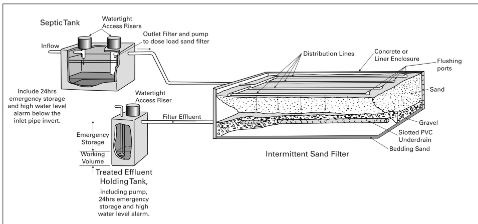
Figure 4.3 Example Of An intermittent Sand Filter
