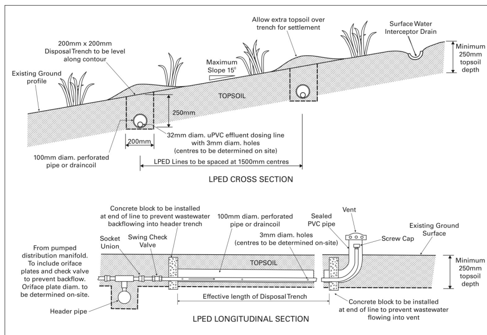
Figure 6.2 Example of a Shallow LPED Land Application System
