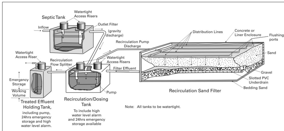
Figure 4.4 Example of a Recirculating Sand Filter
