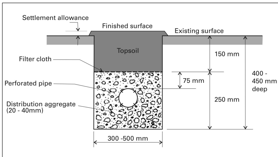
Figure 6.3 Typical Conventional Trench Detail
