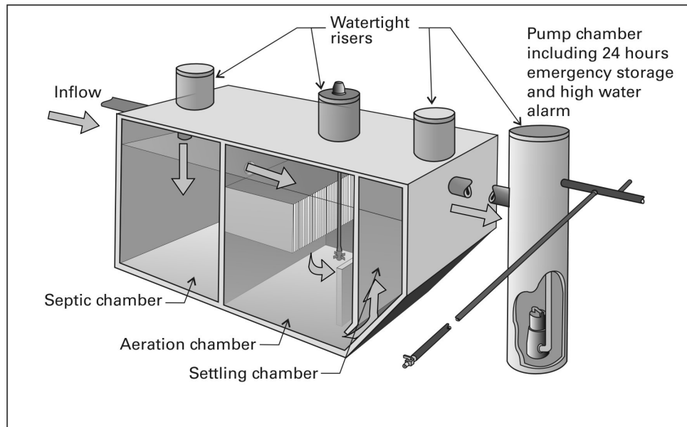
Figure 4.2 Example of An Aerated Wastewater Treatment System
