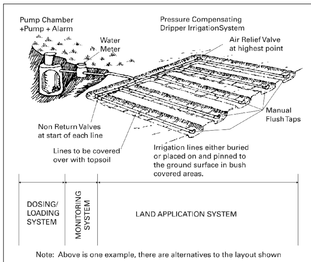
Figure 6.1 Schematic of a Sub-surface pressure Compensating Pressure Compensating Dripper Land Application System
