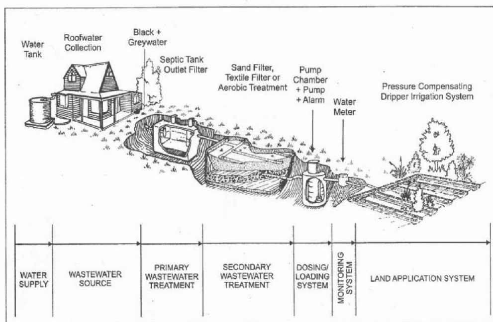
Figure 1.2 Process-flow schematic for on-site wastewater system components. (Source: Auckland Regional Council TP58 2004).
