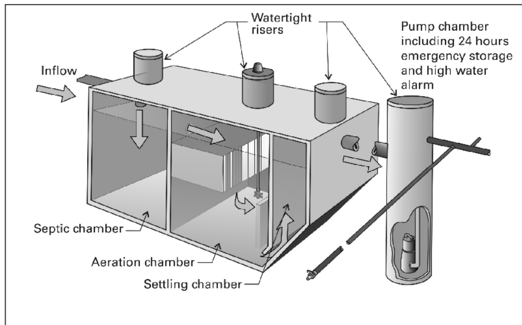
Figure 4.2 Example of An Aerobic Aerated Wastewater Treatment System
