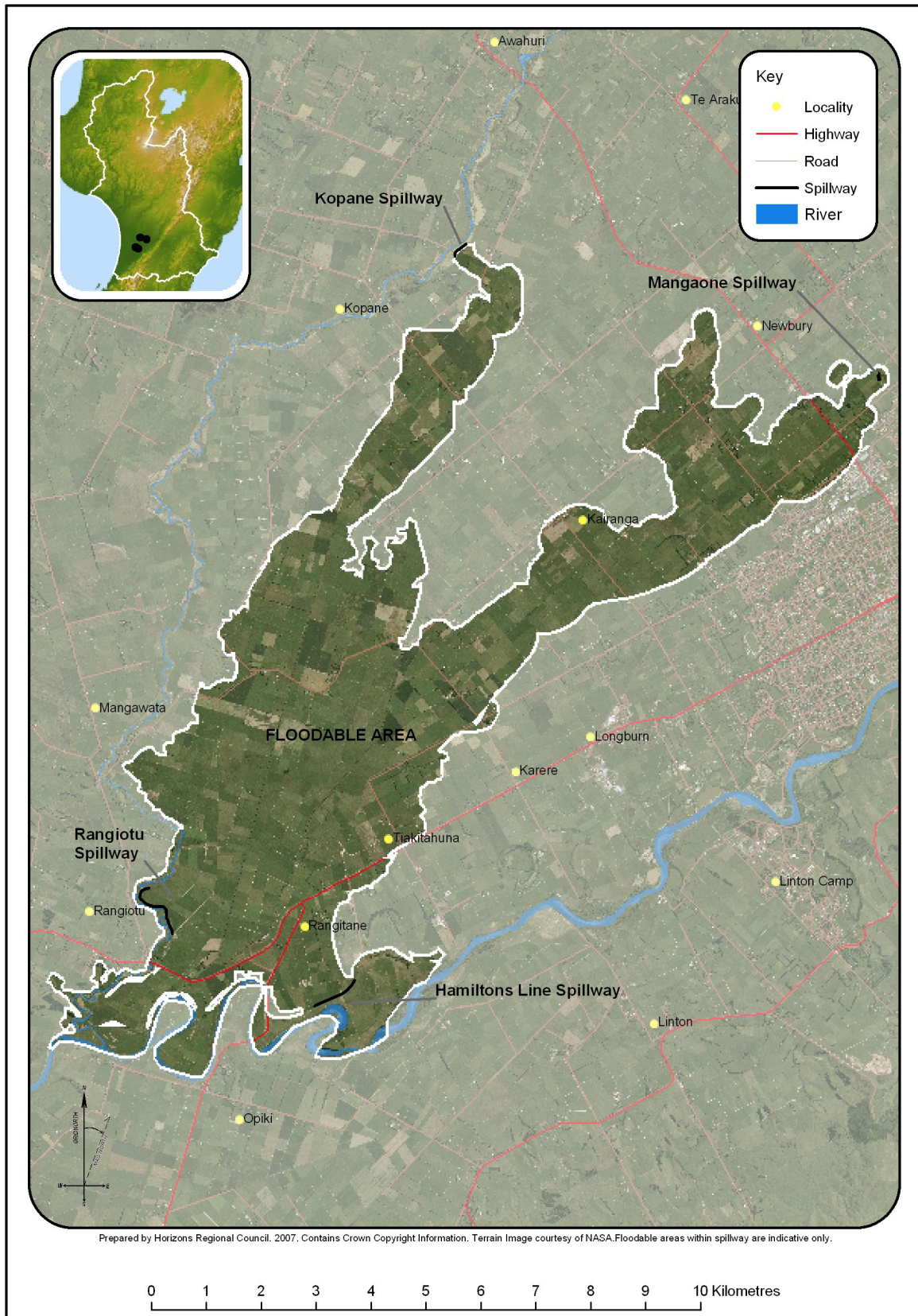
Figure I:3 Taonui Basin Spillway
