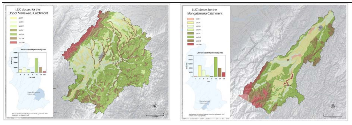
Fig. 20 LUC classes for the Upper Manawatu and Mangatainoka catchments.
