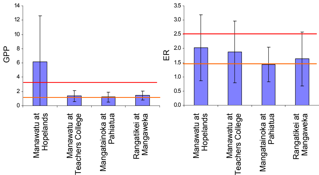
Figure 6. Ratio of rates of GPP and ER ( \text{g O}_2 \text{ m}^{-2} \text{ d}^{-1} ) for four sites on rivers in the Manawatu-Wanganui Region compared to Rangitikei at Onepuhi. Bars show annual means and standard deviations. Horizontal lines mark absolute values used to assess ecosystem health from Young et al. (2008): below the orange line is ‘healthy’, above the orange line is ‘satisfactory’ and above red line is ‘poor’.
