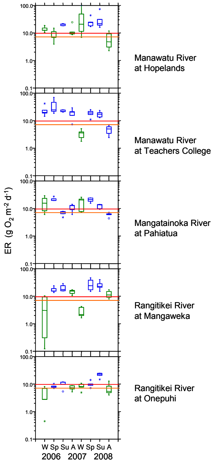
Figure 4. Rates of ecosystem respiration (ER) for five study sites on rivers in the Manawatu-Wanganui Region. Box plots show the median, upper and lower quartiles and range of values. Green boxes indicate ER calculated using corrected data. Horizontal lines mark absolute values used to assess ecosystem health from Young et al. (2008): below the orange line is 'healthy', above the orange line is 'satisfactory' and above red line is 'poor'. Note Y axis is on a log 10 -scale.
