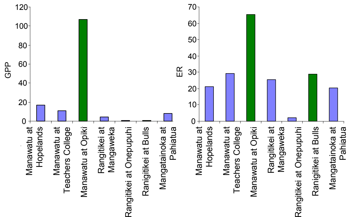
Figure 7. Rates of GPP and ER ( \text{g O}_2 \text{ m}^{-2} \text{ d}^{-1} ) for seven sites on rivers in the Manawatu-Wanganui Region on 27 November 2007. Green bars indicate sites measured as part of another study.
