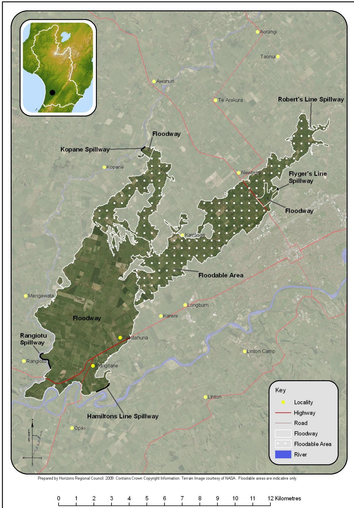
Figure I:3A Taonui Basin spillways, floodways and floodable areas
