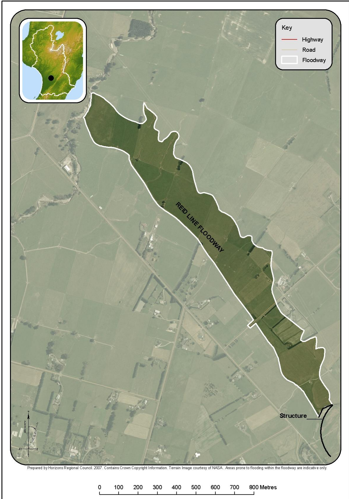
Figure I:4A Reid Line floodway
