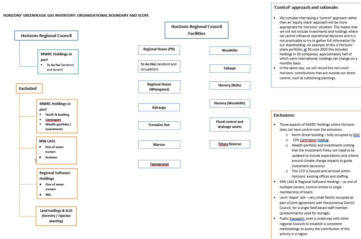
Figure 5: Organisational structure
