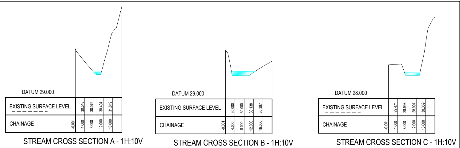
INDICATIVE 100-YEAR ARI WATER LEVELS IN TRIBUTARY DOWNSTREAM OF COLEY POND
