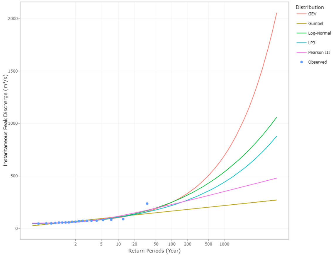
Station 33149 L-moments Fitted Frequency Distributions
