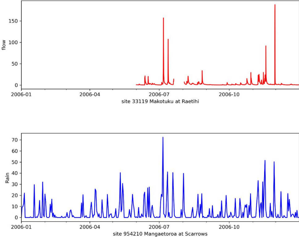
Figure 2-3: Example of gaps in flow records. Annual flow record (top) with gaps, and comparison with rainfall (bottom).
