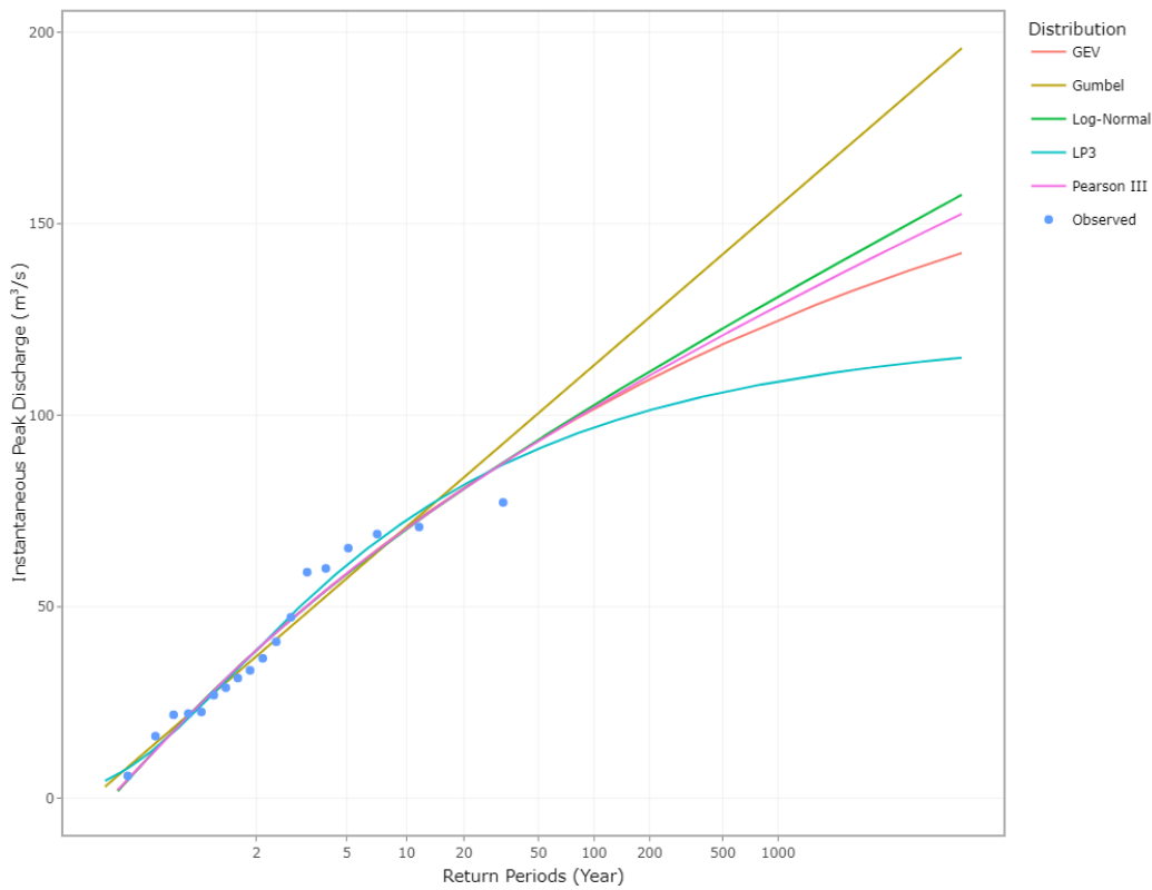
Station 1232563 L-moments Fitted Frequency Distributions
