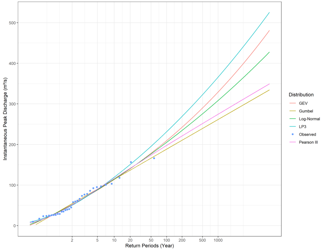
Station 1132523 L-moments Fitted Frequency Distributions
