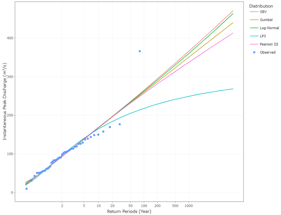
Station 2232510 L-moments Fitted Frequency Distributions
