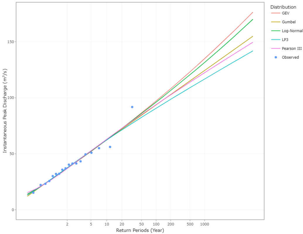
Station 1232581 L-moments Fitted Frequency Distributions
