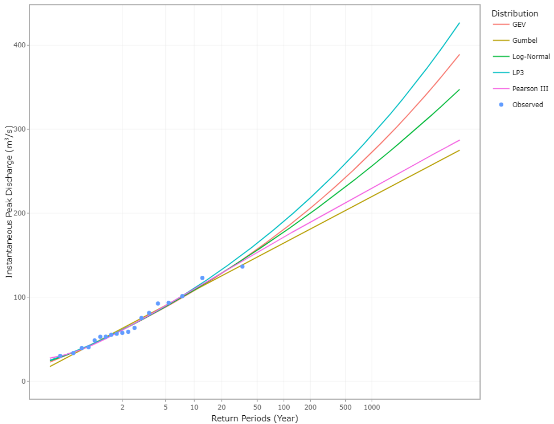
Station 1132519 L-moments Fitted Frequency Distributions
