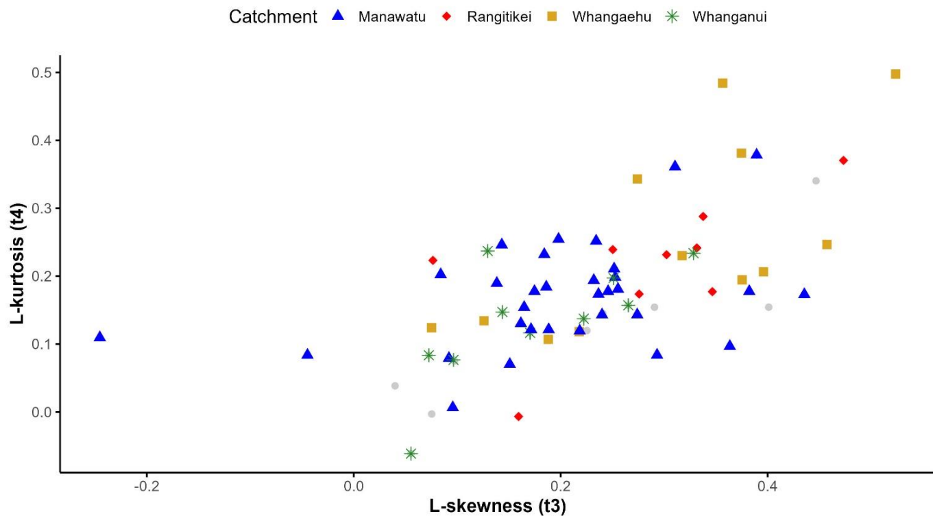
Figure 4-2: HRC L-moment ratios by four major catchments.
