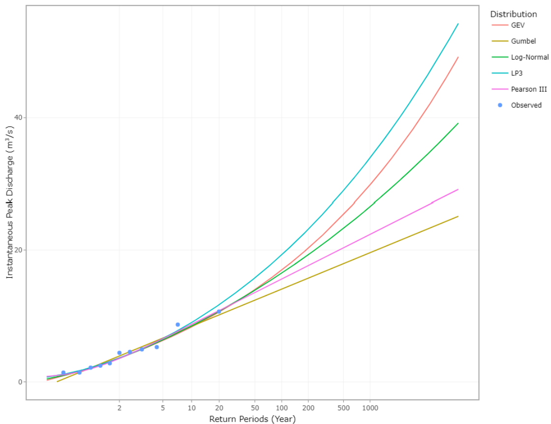
Station 32302 L-moments Fitted Frequency Distributions
