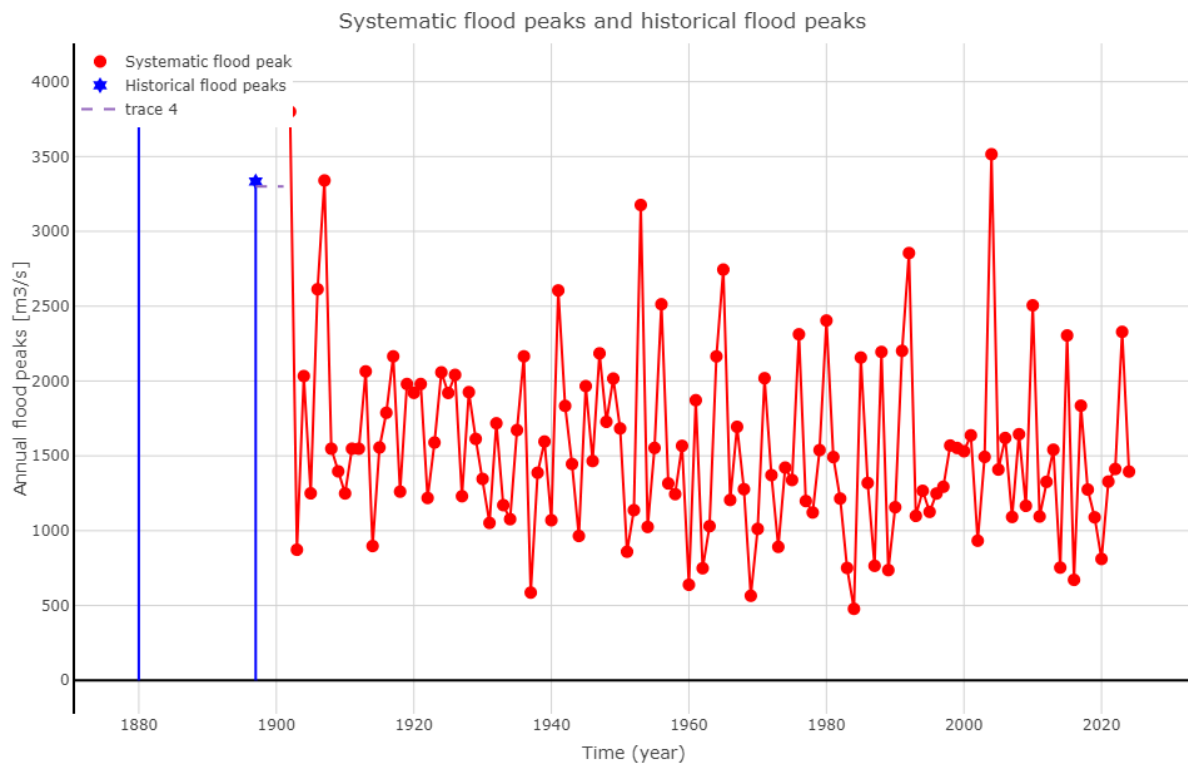
Figure XX-2: Historical information and systematic records.
