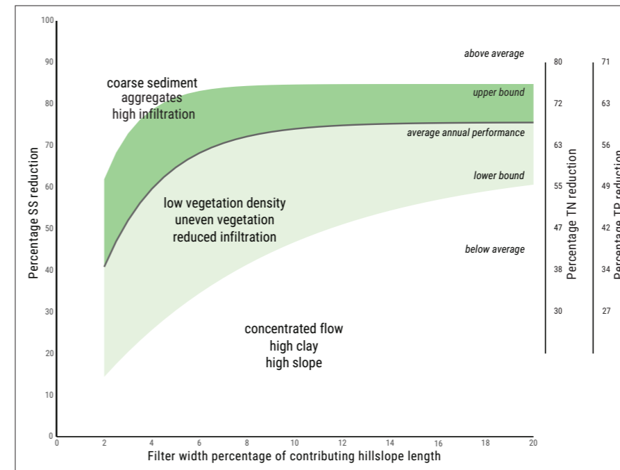
Figure 7. Long-term median annual reduction of suspended sediment (SS), total nitrogen (TN) and total phosphorus (TP) with local condition adjustments. Applicable to areas without clay soils (<28.5% clay content) and low to gently rolling slopes (<11 degrees). The solid line shows expected long-term average performance, with shaded ± 95% confidence intervals.
